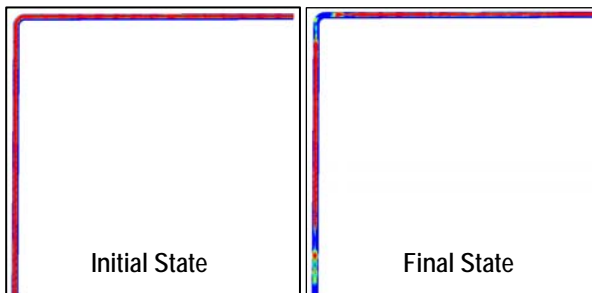
CFD model results showing the resulting pressure within the pipeline as a result of a pressure pulse at the inlet.
